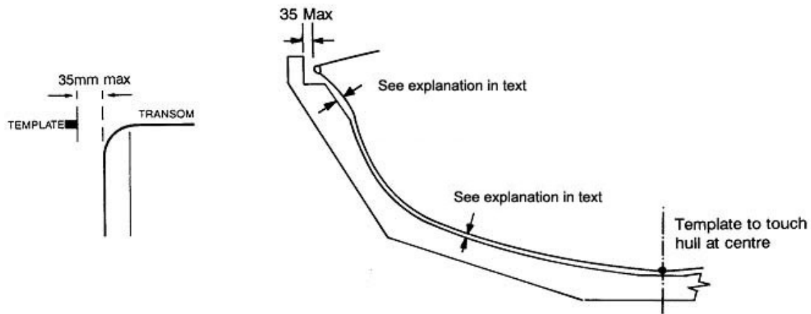
Hull Profile
